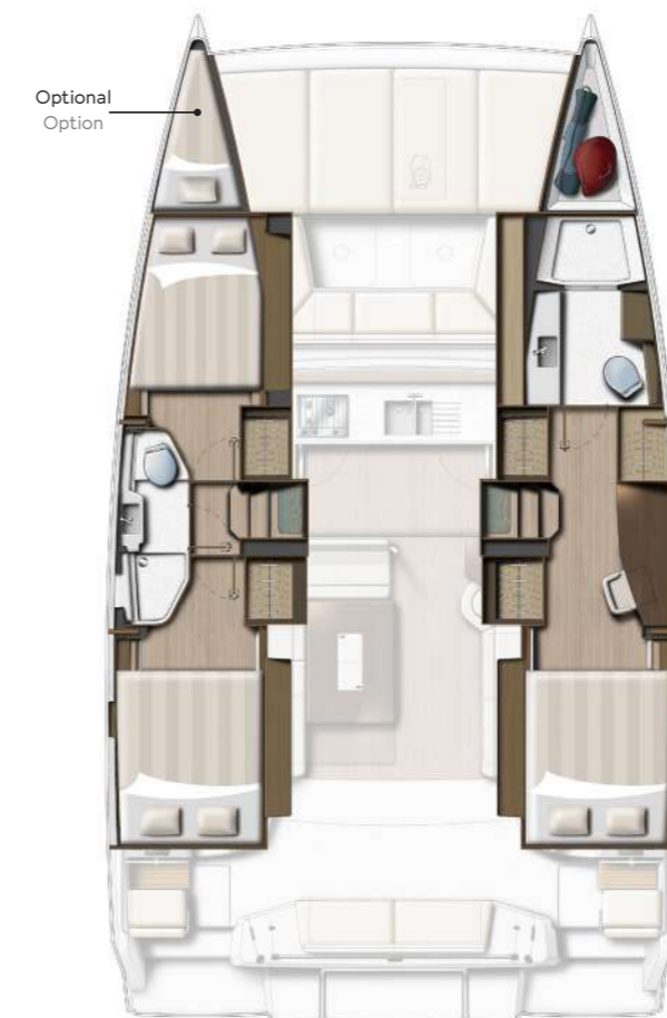
3 DOUBLE CABINS / 2 HEADS VERSION VERSION 3 CABINES DOUBLES / 2 SDB
