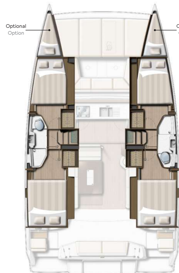
4 DOUBLE CABINS / 2 HEADS VERSION VERSION 4 CABINES DOUBLES / 2 SDB
